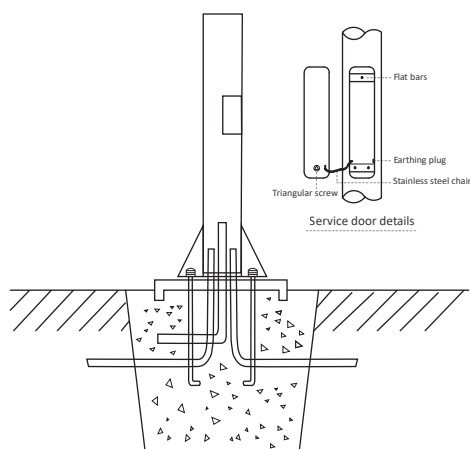
Access door & grounding
